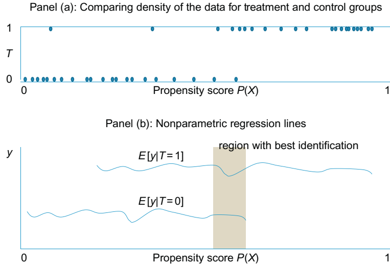
Figure 1.2 Schematic diagrams for matching estimators.
